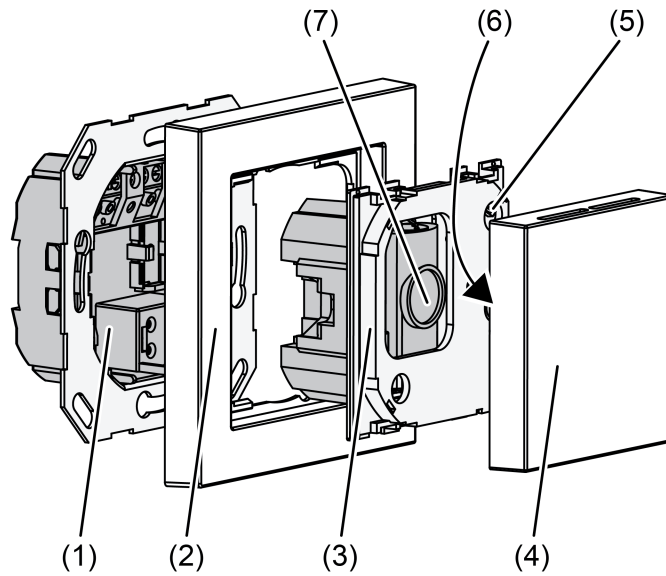
Figure 1: Device components CO 2 Sensor
