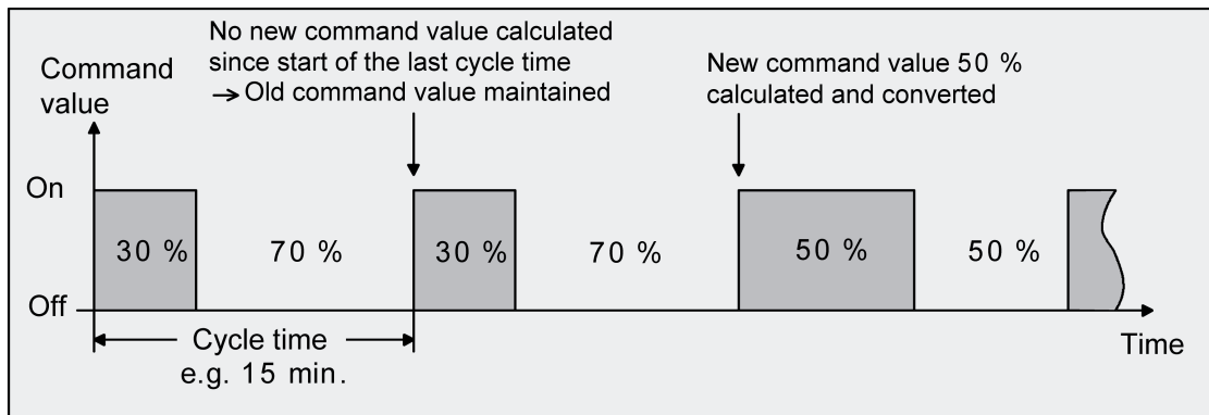
Figure 19: Switching PI control
