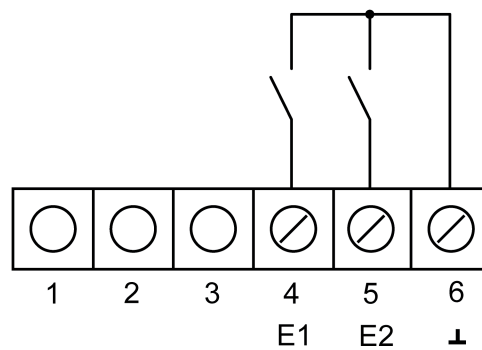
Figure 4: Connection of binary inputs
