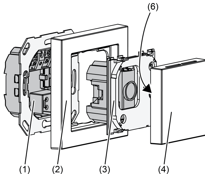
Figure 2: Device fitting
