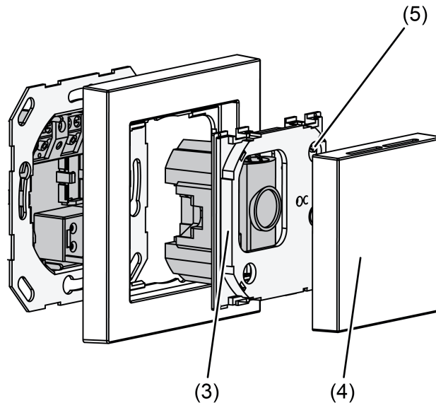
Figure 6: Location of the programming button and LED
