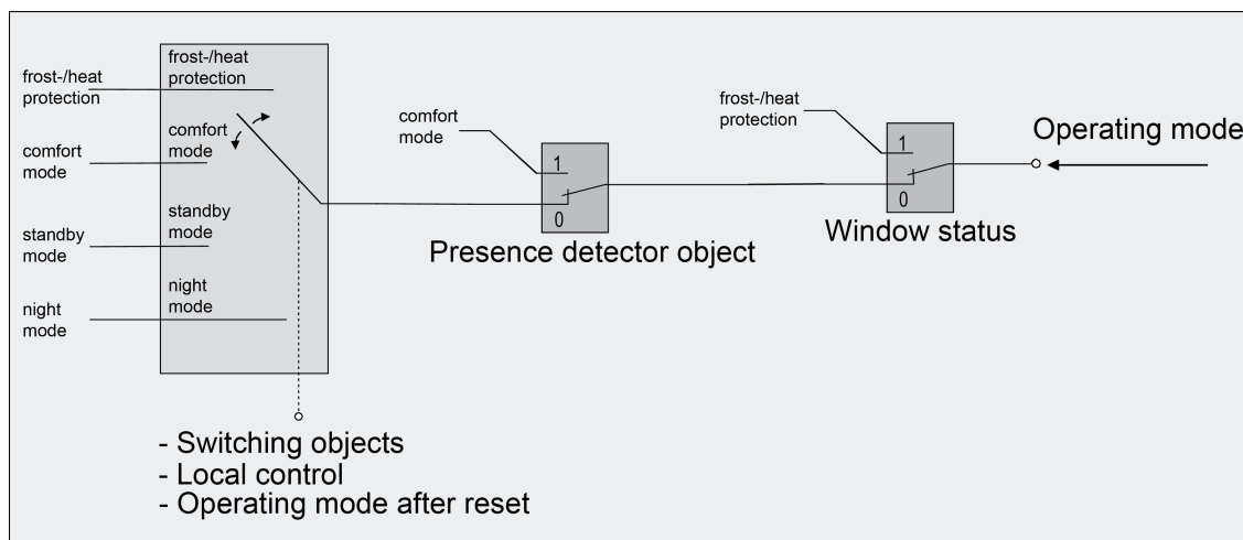
Figure 27: Operating mode change-over through 4 x 1-bit objects with motion detector
