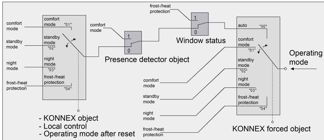
Figure 29: Operating mode change-over through KONNEX object with motion detector
