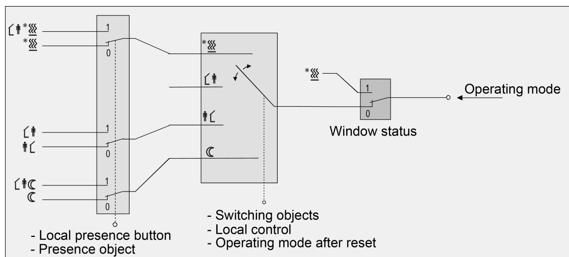
Figure 35: Operating mode change-over through 4 x 1-bit objects with presence button
