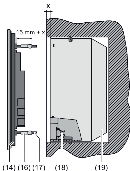
Figure 4: Device mounting of a TS Comfort glass sensor
