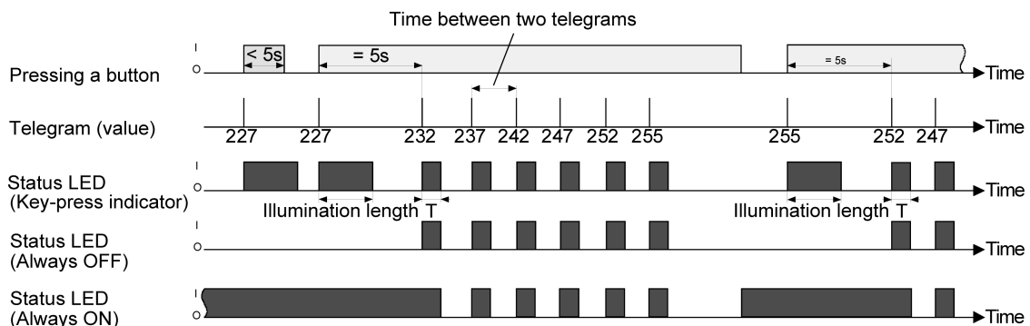
Figure 22: Example of value adjustment without value range overflow
