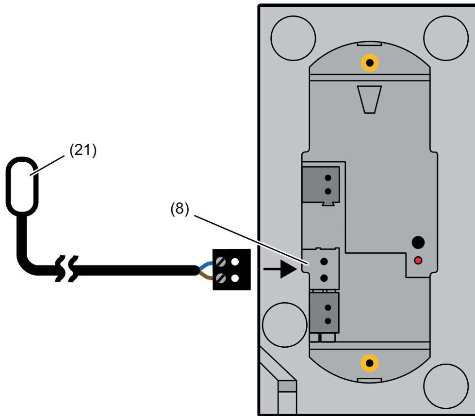
Figure 47: Connection for wired temperature/remote sensor
