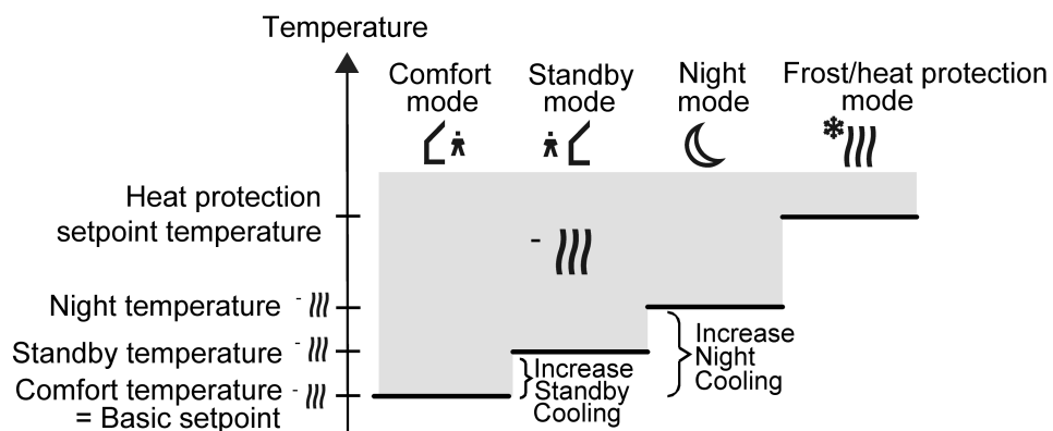
Figure 41: Setpoint temperatures in the operating mode "Cooling" (recommended specification)
