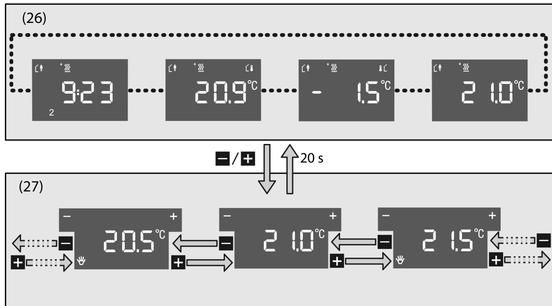
Figure 8: Basic setpoint shift using display buttons
