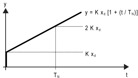
Figure 33: Function of the command value of a PI control
