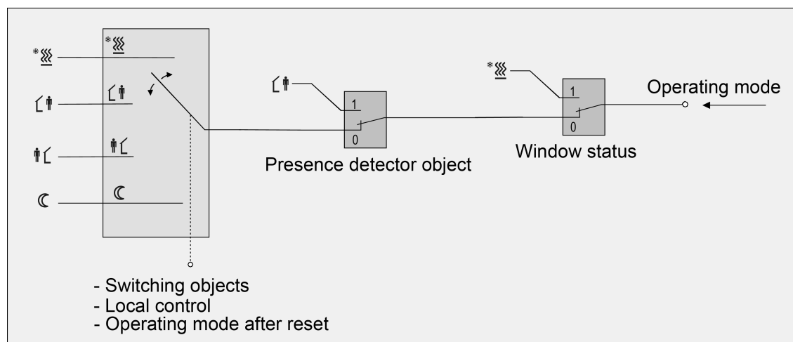
Figure 36: Operating mode change-over through 4 x 1-bit objects with motion detector
