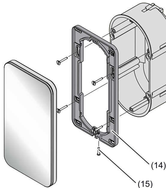
Figure 3: Device fitting
