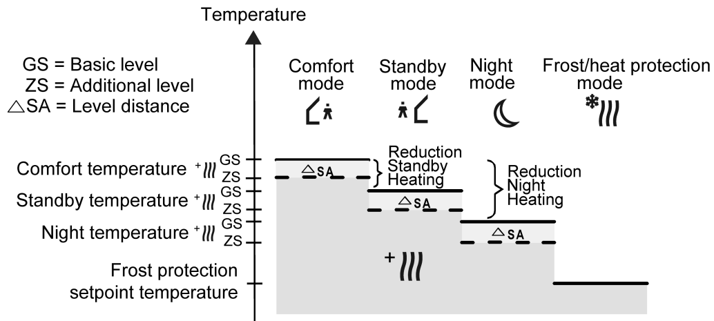
Figure 40: Setpoint temperatures in the operating mode "Basic and additional heating" (recommended specification)
