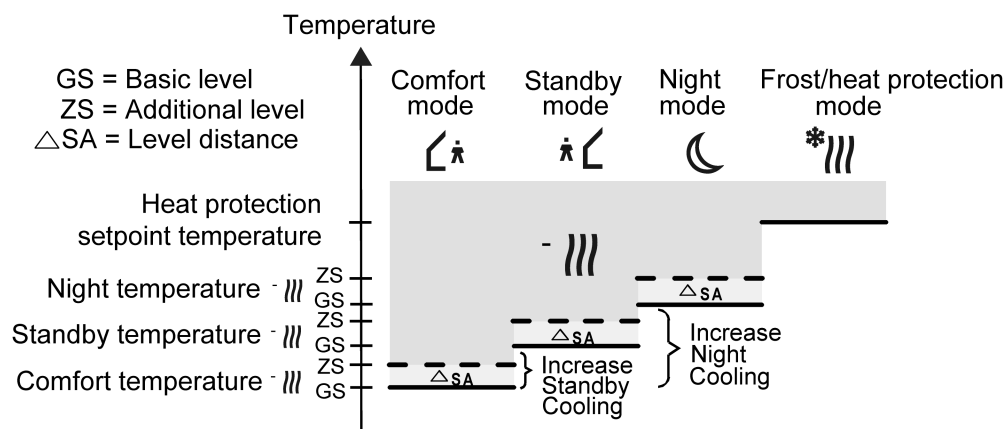
Figure 42: Setpoint temperatures in the operating mode "Basic and additional cooling" (recommended specification)
