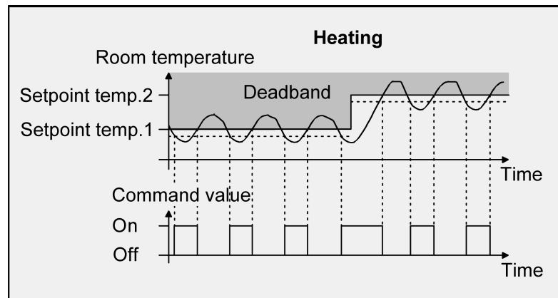
Figure 31: 2-point feedback control for mixed "Heating and cooling" mode with active heating mode.
