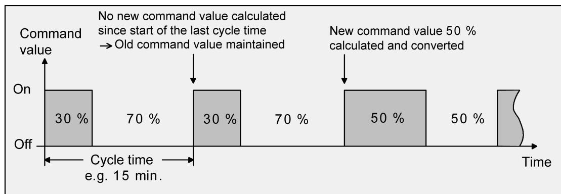
Figure 28: Switching PI control
