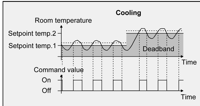
Figure 32: 2-point feedback control for mixed "Heating and cooling" mode with active cooling operation.
