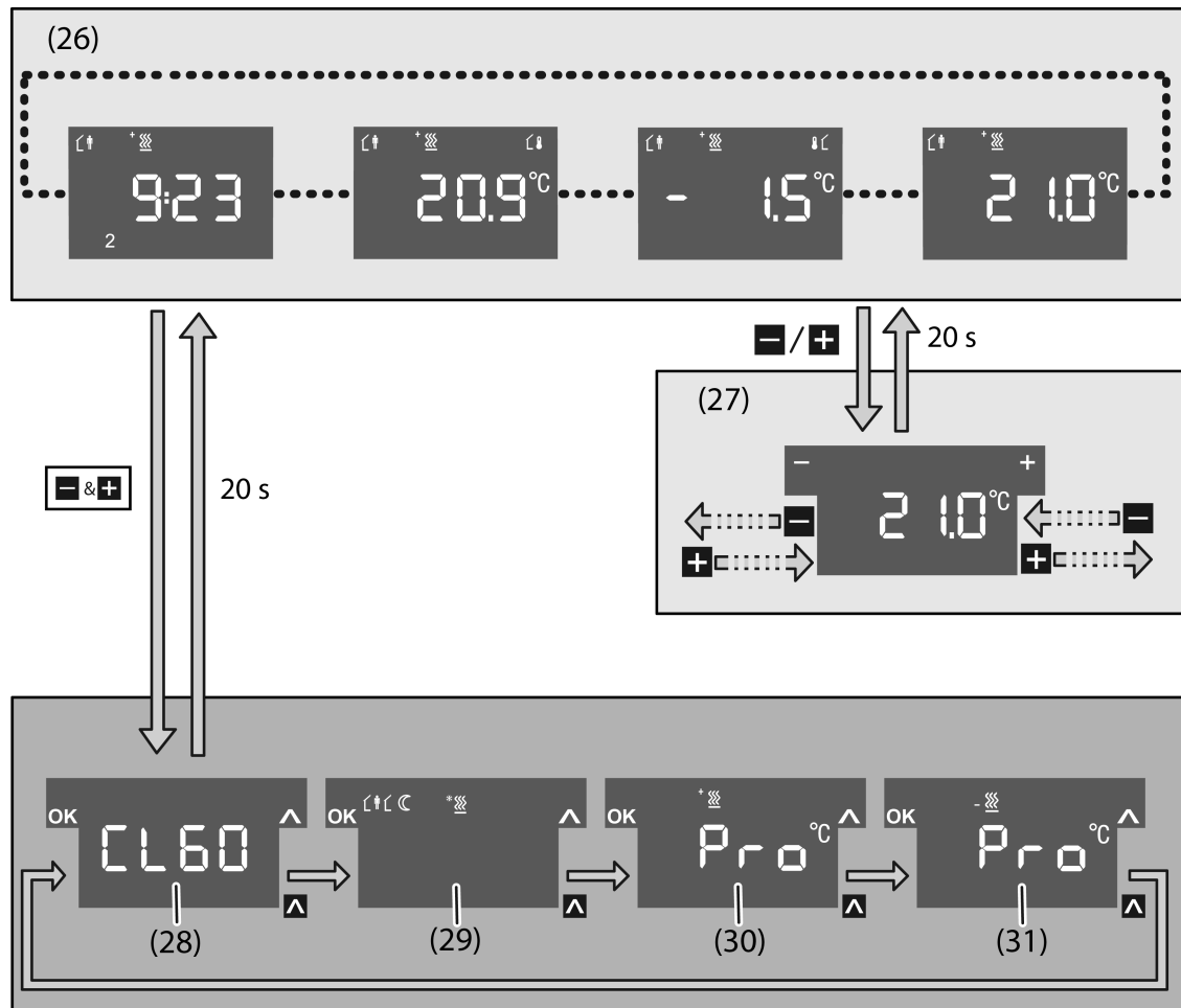
Figure 9: Main menu of the second operating level
