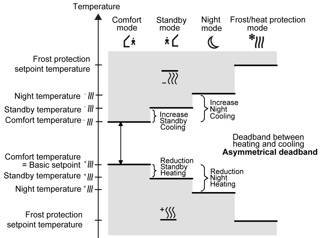
Figure 44: Setpoint temperatures in the operating mode "Heating and cooling" with asymmetrical deadband (recommended specification)
