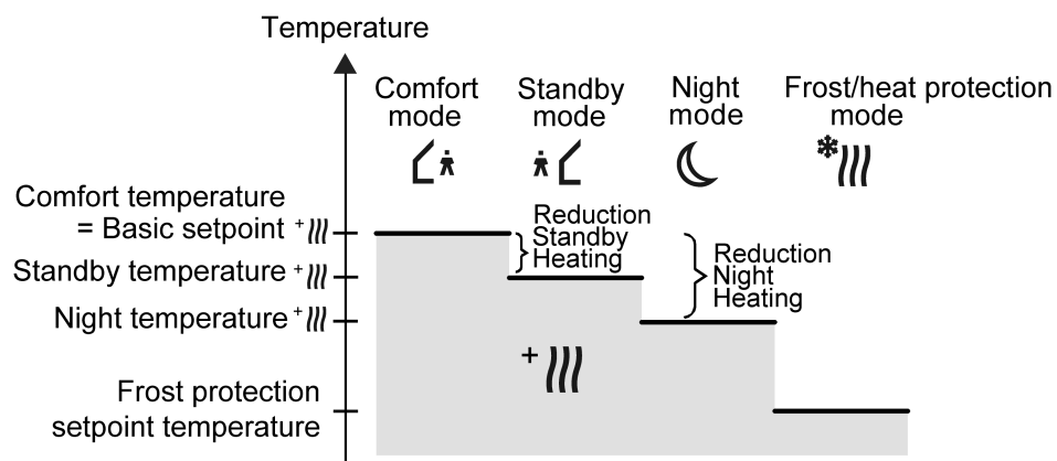
Figure 39: Setpoint temperatures in the operating mode "Heating" (recommended specification)
