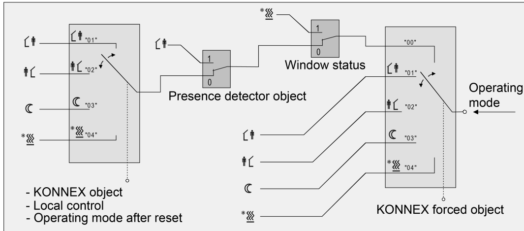
Figure 38: Operating mode change-over through KONNEX object with motion detector
