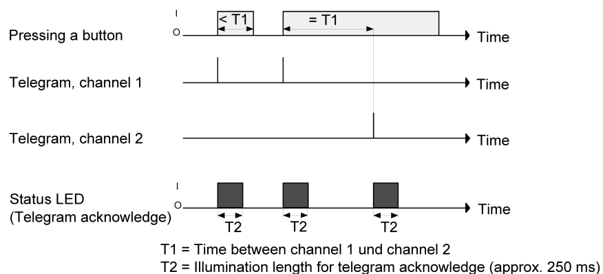
Figure 25: Example for operation concept "Channel 1 and channel 2"
