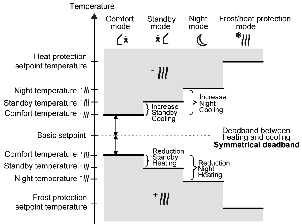
Figure 43: Setpoint temperatures in the operating mode "Heating and cooling" with symmetrical deadband (recommended specification)
