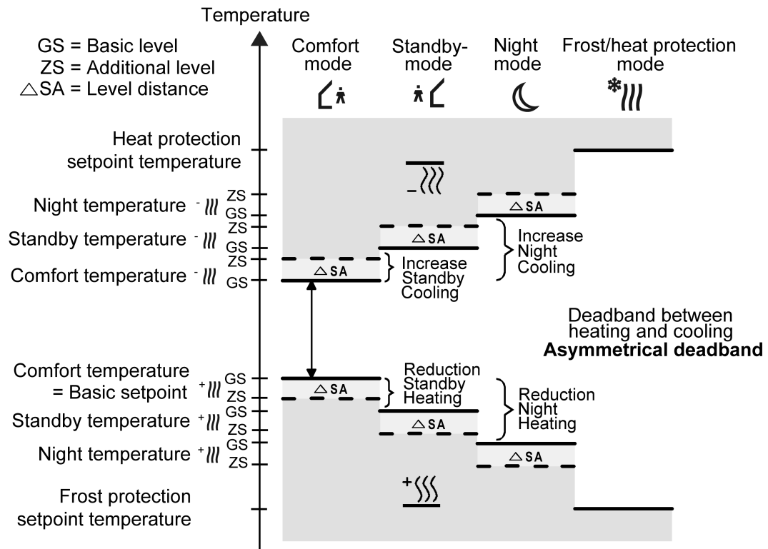
Figure 46: Setpoint temperatures in the operating mode "Basic and additional heating and cooling" with asymmetrical deadband (recommended specification)
