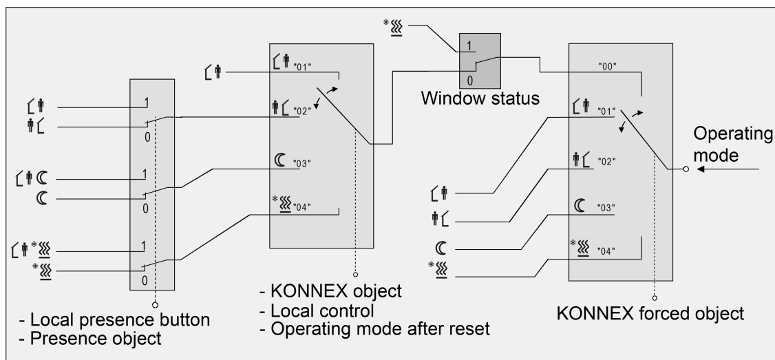
Figure 37: Operating mode change-over through KONNEX object with presence button
