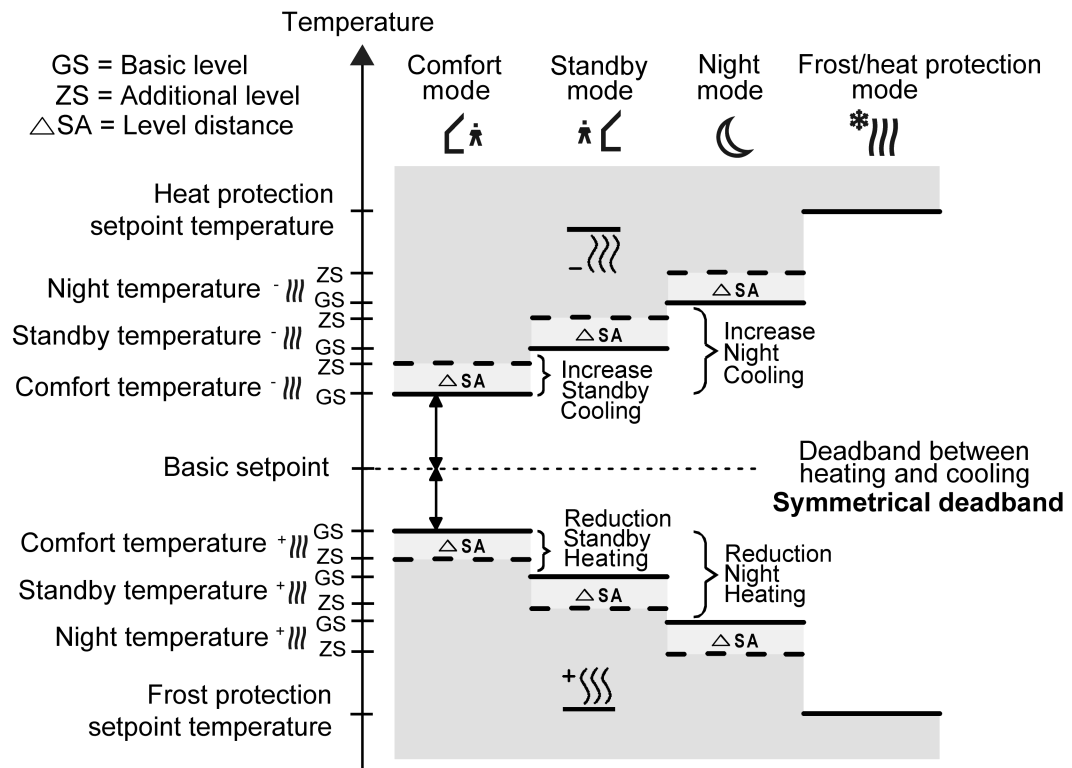
Figure 45: Setpoint temperatures in the operating mode "Basic and additional heating and cooling" with symmetrical deadband (recommended specification)
