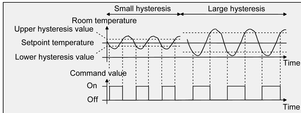
Figure 34: Effects of the hysteresis on the switching behaviour of the command value of 2-point feedback control
