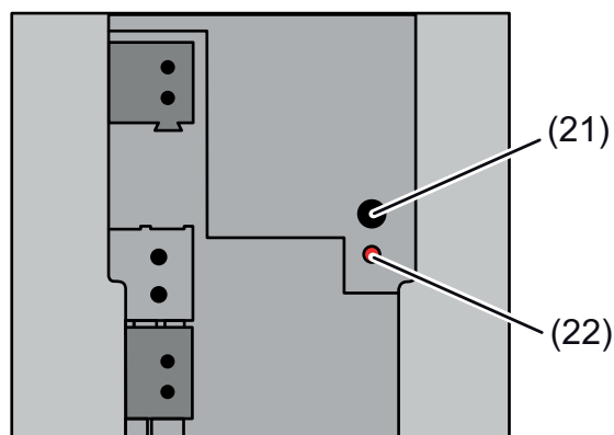
Figure 6: Programming buttons and LED on the rear side of the device
