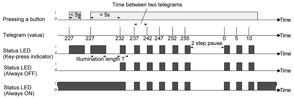
Figure 23: Example of value adjustment with value range overflow
