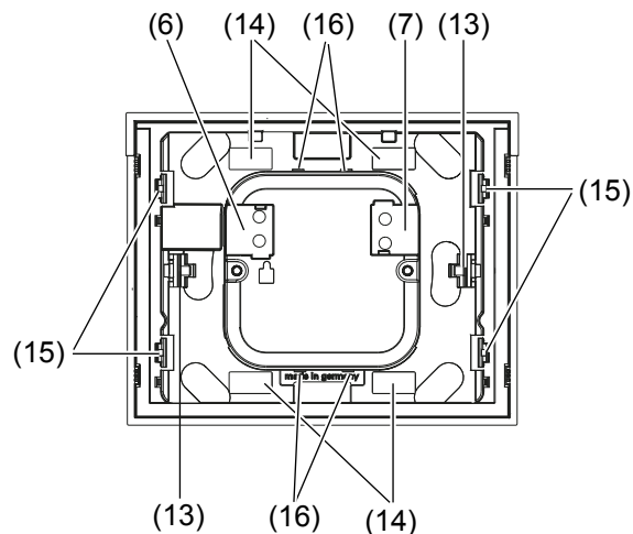
Figure 11: Rear view
