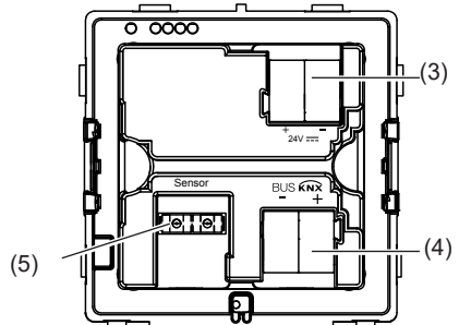
Figure 2: Rear view
