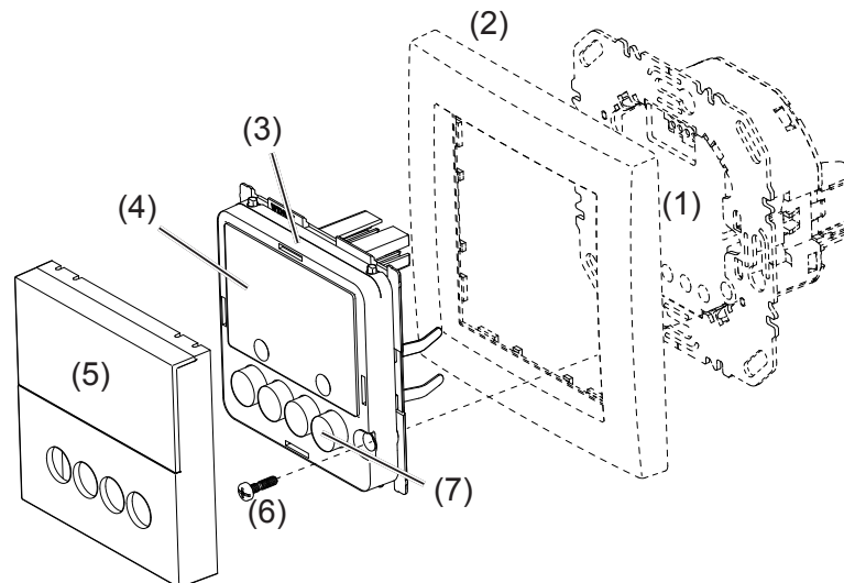
Figure 1: Design and layout of the device
