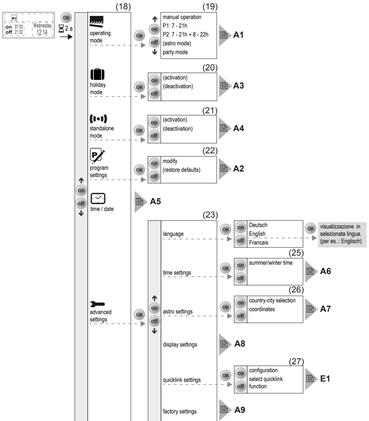
Figure 4: Menu overview
