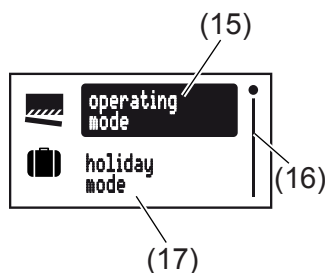
Fig. 3: Main menu
