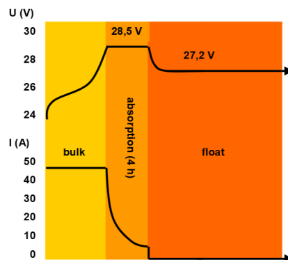
Charge curve
