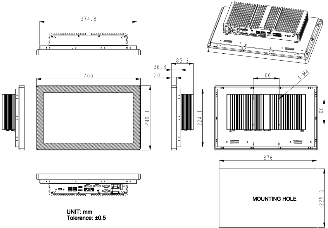
Figure 1.1: Dimensions of NPP-156P01
