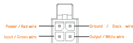
Power socket pinout
