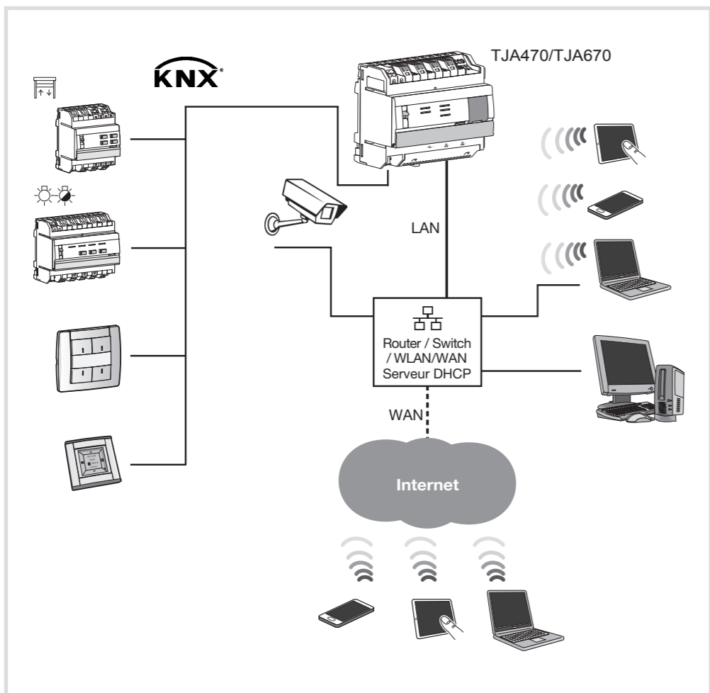
Picture 2: the server and its environment
