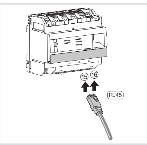
Picture 3: connection to the IP network
