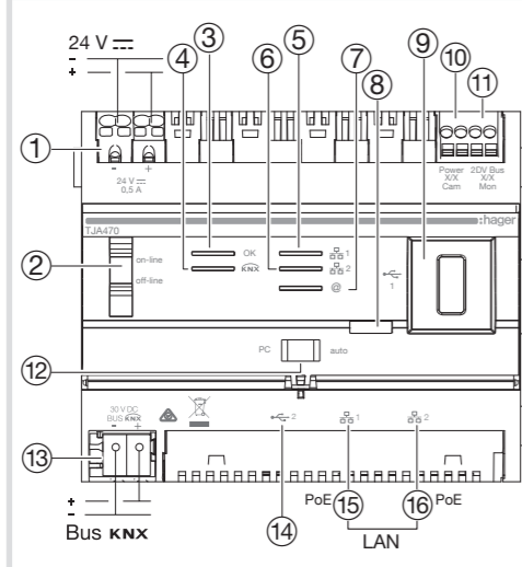
Picture 1: device components
