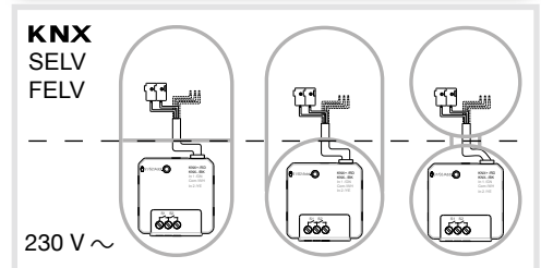
Figure 2: installation with separate terminal compartment
