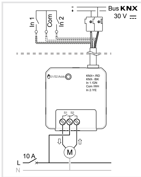
Figure 4: connection of motors
