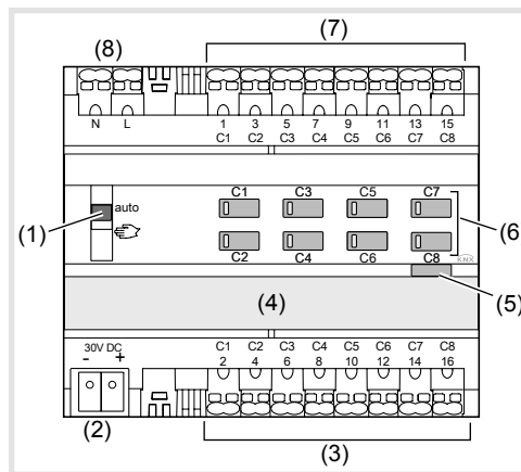
Fig. 1: Example device variant 8/4gang
